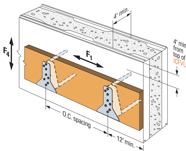
Typical Wood Ledger Installation with ICFVL8
