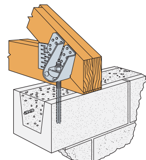
Typical VGT Installation
