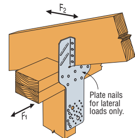
H10S Installation with Stud Offset
