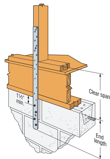
Typical MSTAM36 Installation
