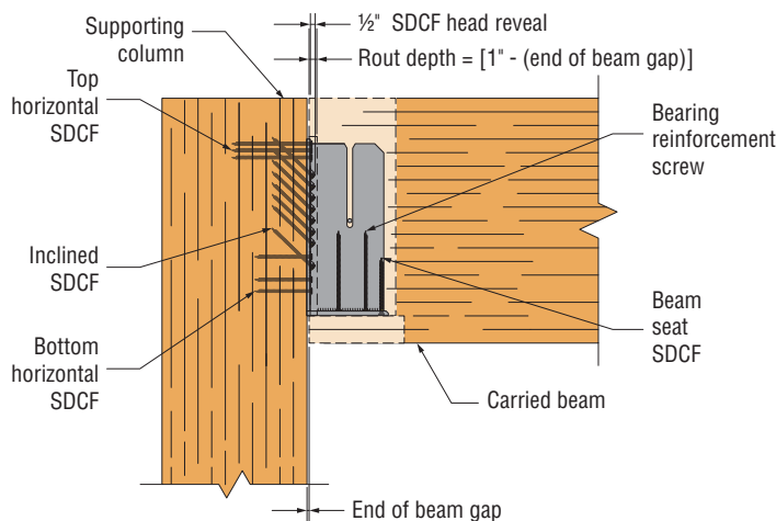
Typical Beam-to-Column Installation
