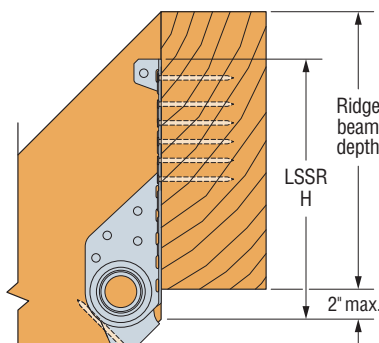
LSSR Installation on Minimum Depth Beam
