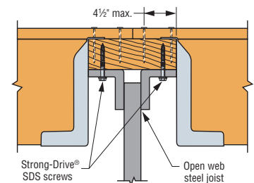
Double HF26N Nailers Installation on Hybrid Truss
