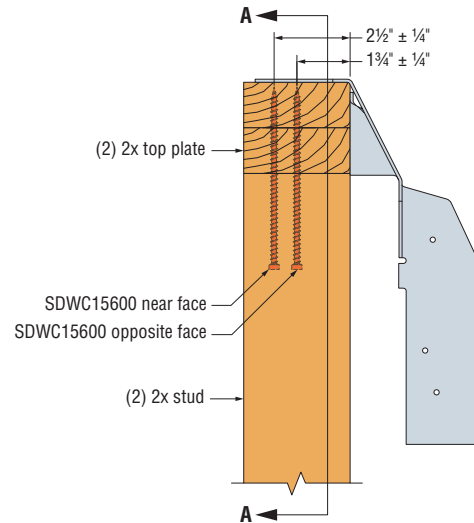
DGHT (over studs with SDWC™)
