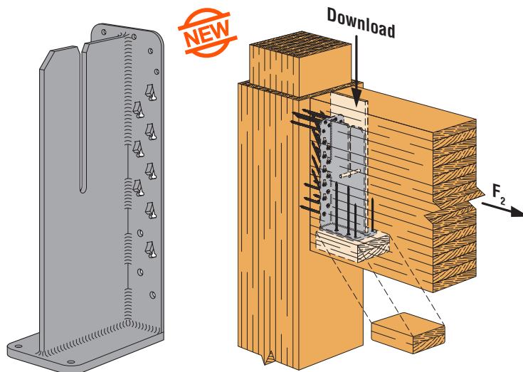
Typical HSKP Installation
