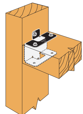
Typical APRTR Installation
