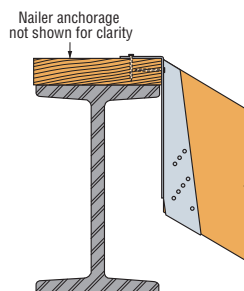
Typical Sloped Down on Nailers Non-Backed
