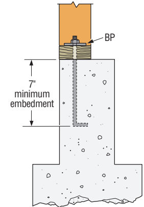
Typical BP Installed with a Muddsill Anchor Bolt
