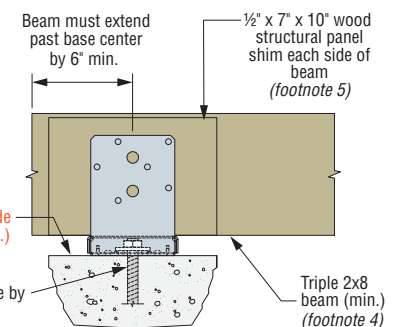
ABU66Z Beam Installation
