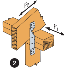
H2A Installation
