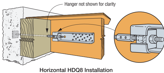
Horizontal HDQ8 Installation
