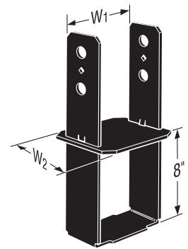
CBPC Classic (see pp. 80–81 for model no. and allowable loads)
