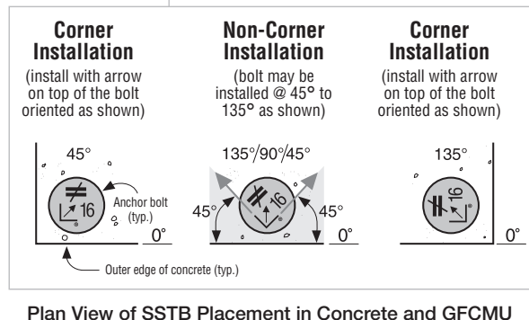
Plan View of SSTB Placement in Concrete and GFCMU
