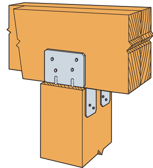
Typical LPC4Z Installation
