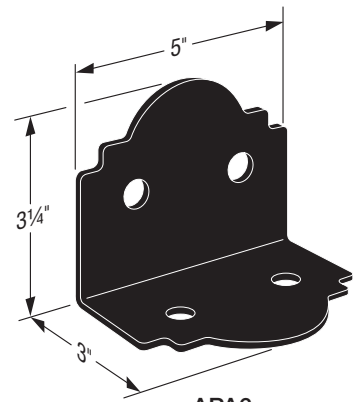
APA6 (others similar) US Patent Pending
