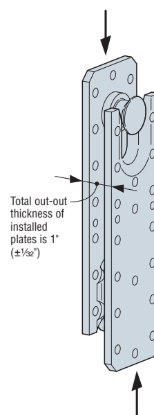
Assembly Thickness and Fit-Up Tolerance
