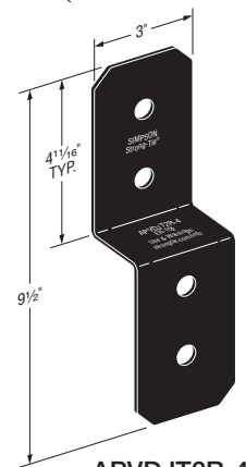
APVDJT2R-4 (others similar)
