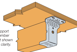
Typical HF24N Installation (HF34N similar)
