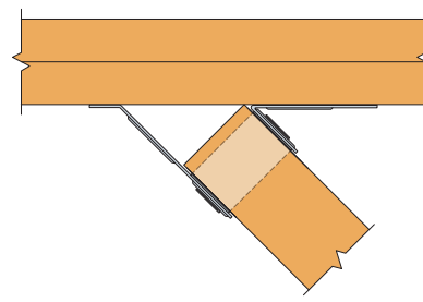
Alternate LSSR Installation (plumb cut)
