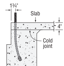
Two-Pour Installation
