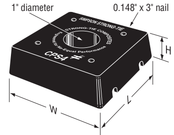
CPS4-R (other sizes similar except CPS46)
