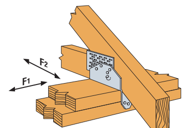
HS24 Installation
