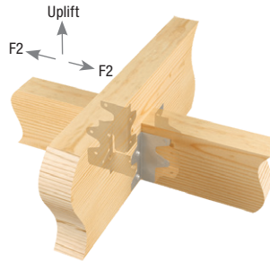
Typical TUS24 installation
