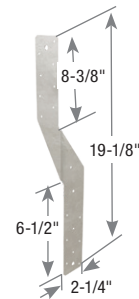
LFTA6 (left version shown)
