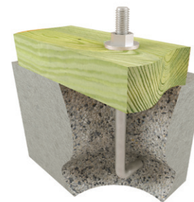
Typical AB128-HDG installation
