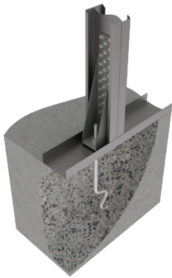
Typical TD10S installation
