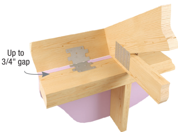
Typical RBC 1" foamboard installation
