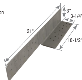
DSC4R right shown
