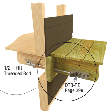
Typical THR deck to ledger installation
