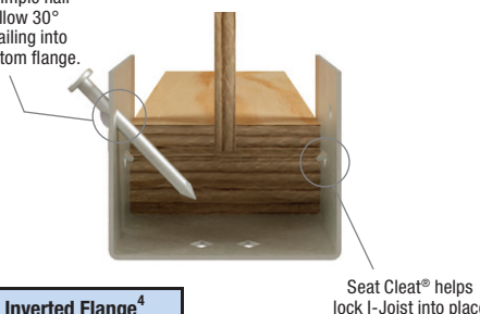
Typical IHF1714 max nailing installation
