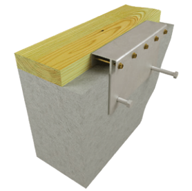
2) Drill and install concrete anchors
