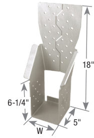
GTQ318 (GTQM318 similar)
