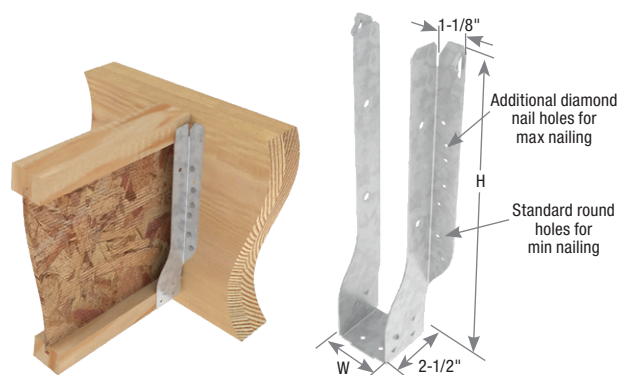
Typical IHFL2514 min nailing installation
