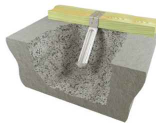
Alternate FA3 installation (concrete slab only)
