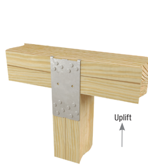
Typical RSPT6-2 installation
