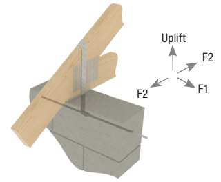
Single HHTA20 roof-truss installation
