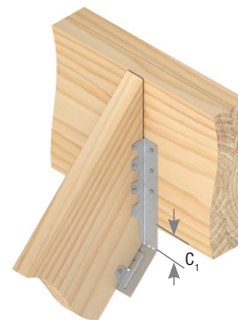
Typical LSRR installation
