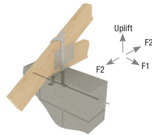
Double HHTA20 roof-truss installation
