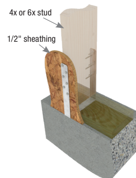
Typical SPTHW installation
