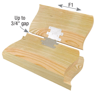
Typical RBC top-plate to inside of blocking installation
