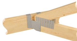
Typical MSH213R installation
