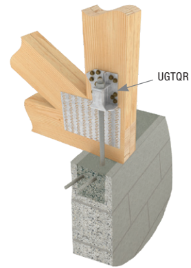
Typical UGTQR masonry installation (right shown)
