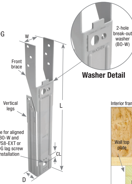
ADTT-TZ out of box
