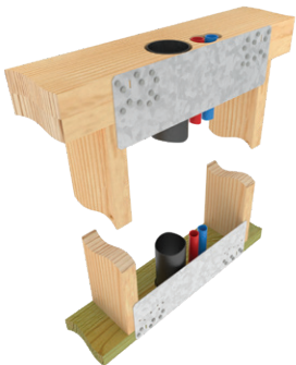
Typical ICPL516-TZ installation
