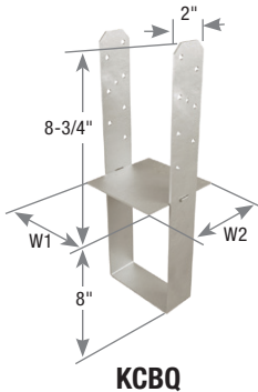
Typical KCBQ installation
