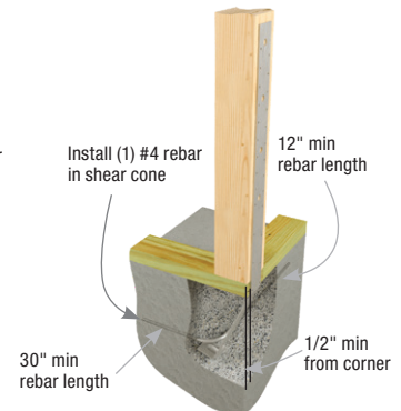
Typical HPAHD22 single pour corner and endwall installation
