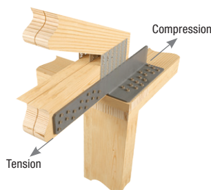
Typical DSC4R installation
