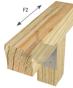
Typical ANJ44S-HDG installation
