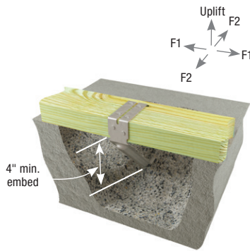
FA3 standard installation in concrete
