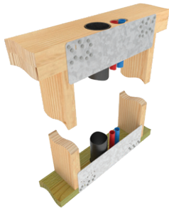
Typical ICPL516-TZ installation
