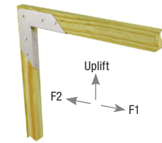
Typical TTA12-TZ installation
