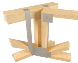
Typical MSHL/R top-min installation
